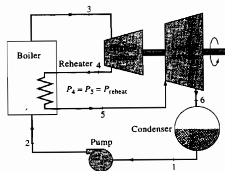
The ideal reheat Rankine cycle.
